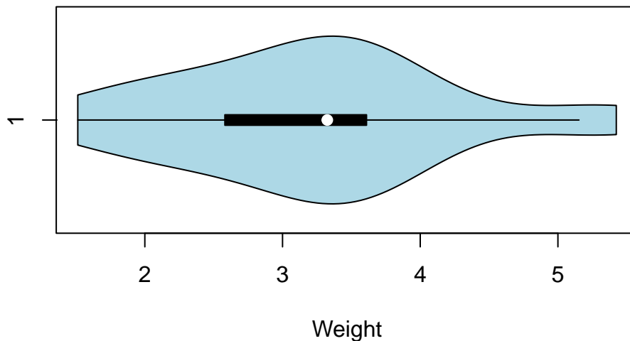
Violin Plot of Weight (wt)
