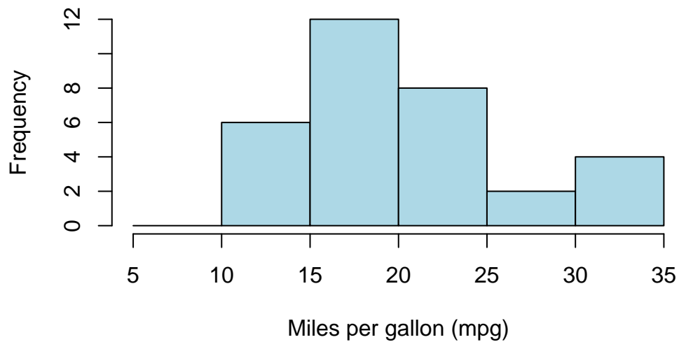
Histogram of Mileage (with breaks of 5)
